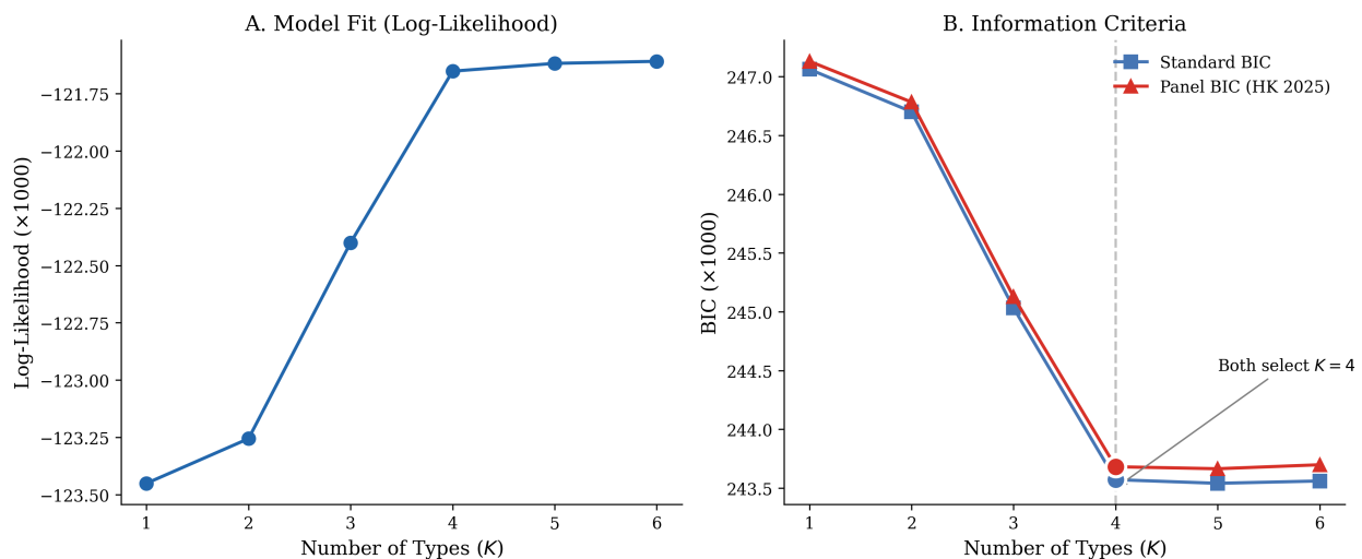
Figure 6: Information Criteria Across K
