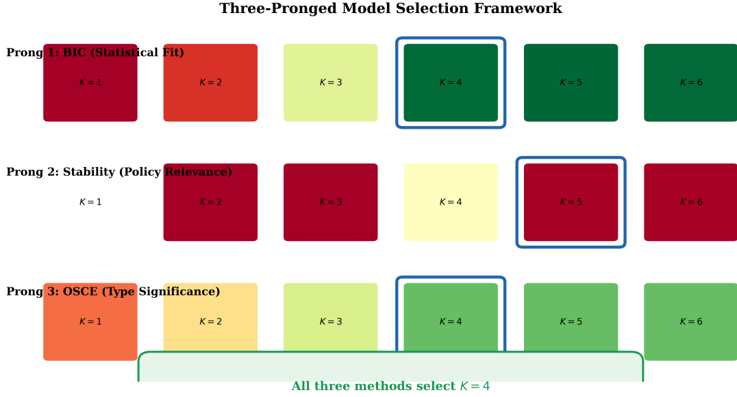
Figure 1: Three-Pronged Model Selection Framework
