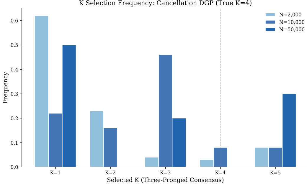
Figure 2: K Selection Frequency: Cancellation DGP (True K = 4 ) Notes: Frequency of selected K (three-pronged consensus) across replications. The true K = 4 is rarely recovered (3–8%), reflecting the fundamental difficulty of separating types under cancellation. The modal selection is K = 1 at N = 2,000 (62%) and K = 3 at N = 10,000 (46%).
